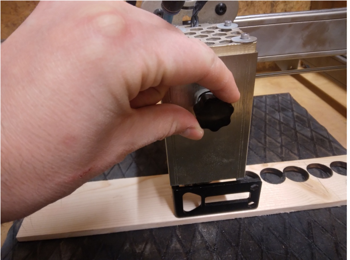
Figure 25: Tighten up the laser again by turning its screw
