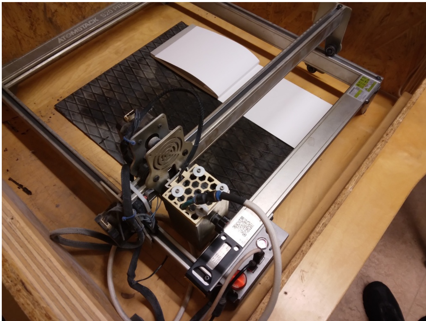
Figure 22: Put the material in the enclosure
